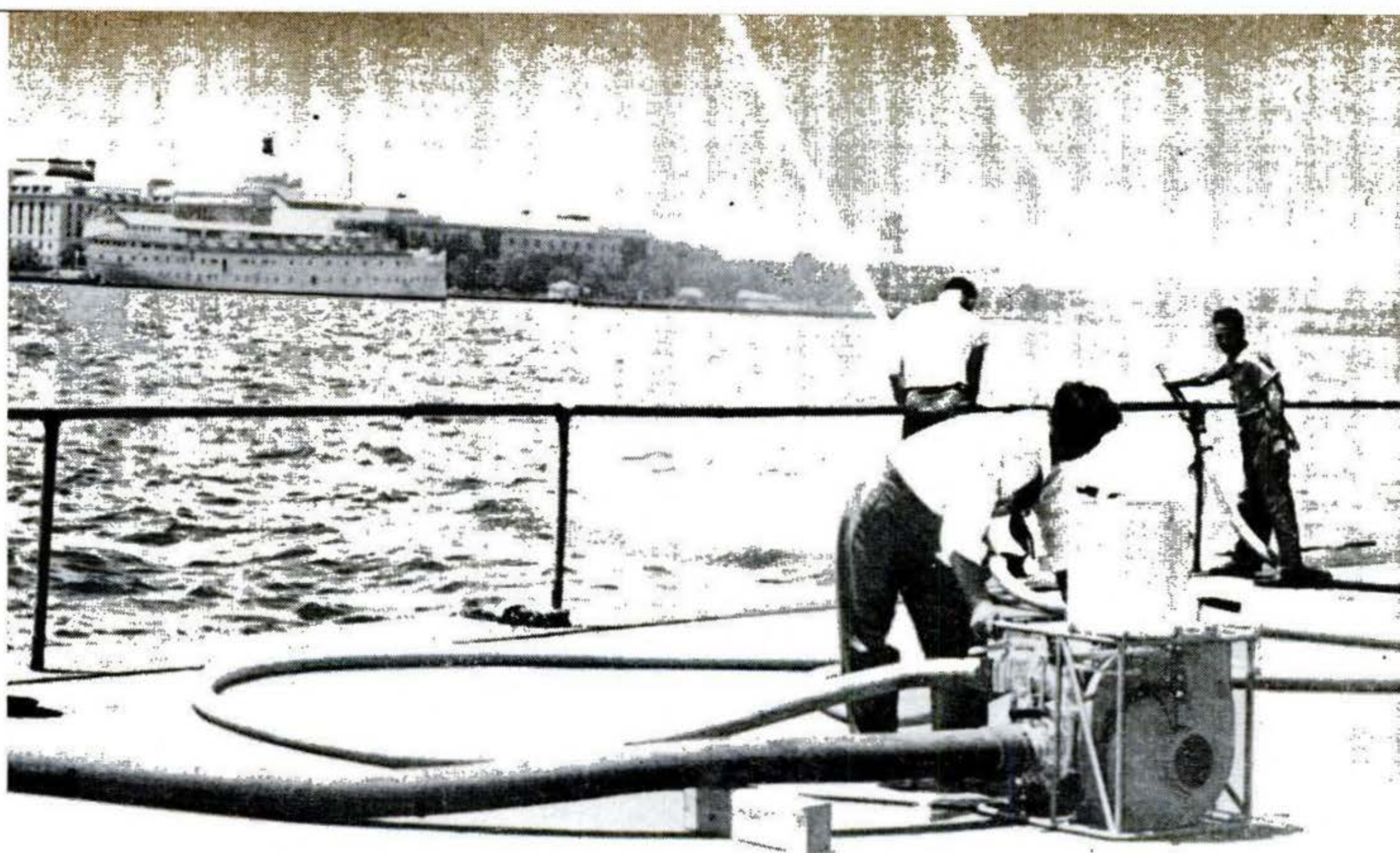
In trials, midget gas-turbine pump delivers 500 gallons of water a minute through two hoses.
